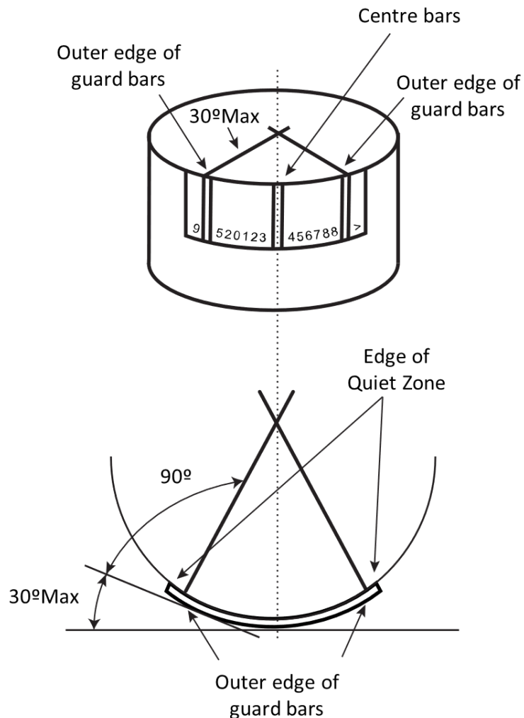
Figure 6.2.3.2-2. Relationship between symbol and curvature
